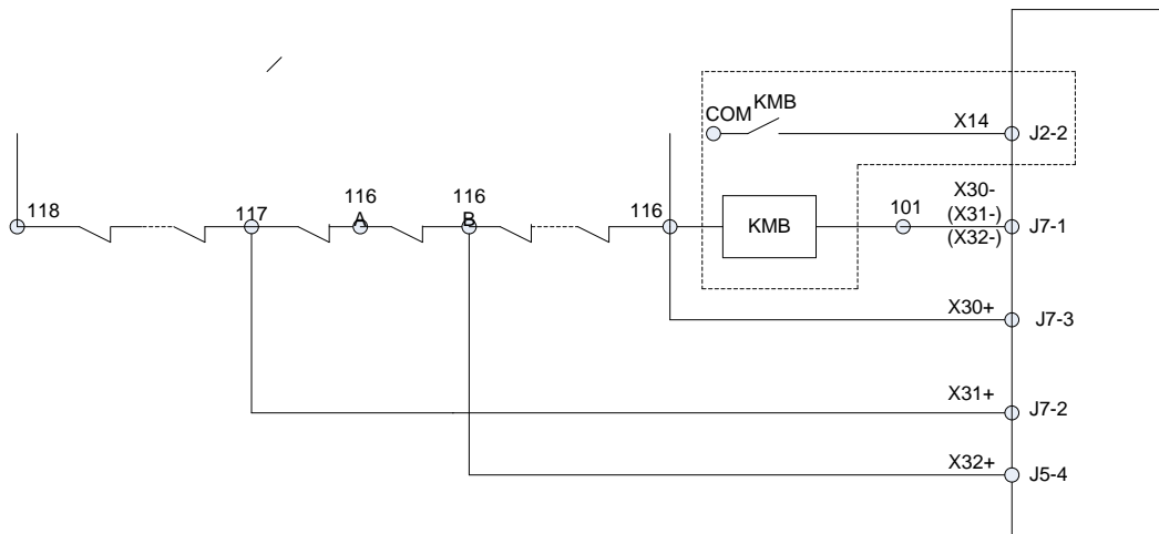
Figure 5 Advance door open & re-leveling & UCMP test & Door short detection control when two
